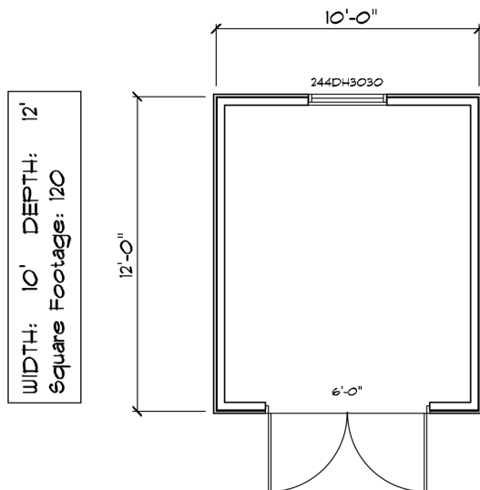
Plan: Goose Creek Shed
